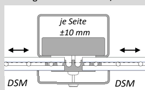
Montagevariante 1: DSM/DSM
