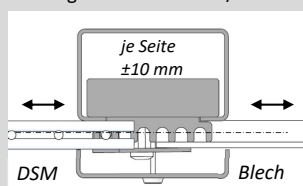
Montagevariante 2: DSM/Blech
